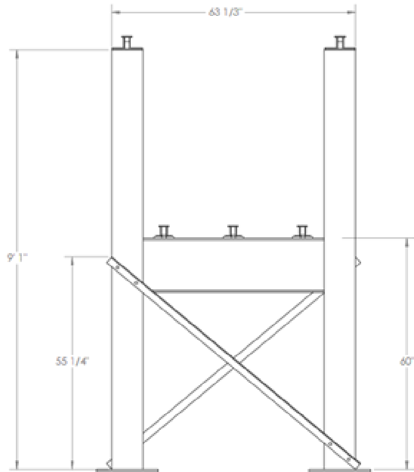
TOWER FRONT VIEW
