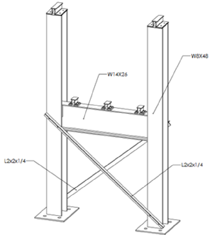
TOWER DIMETRIC VIEW
